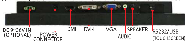
[I/O VIEW] Note: this model is MC121S2-UJBH with DC 9-36V input.
